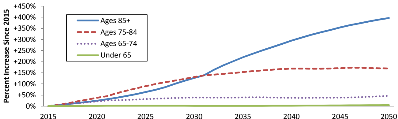
Projected Population Growth in Nevada, by Age Group, 2015-2050
