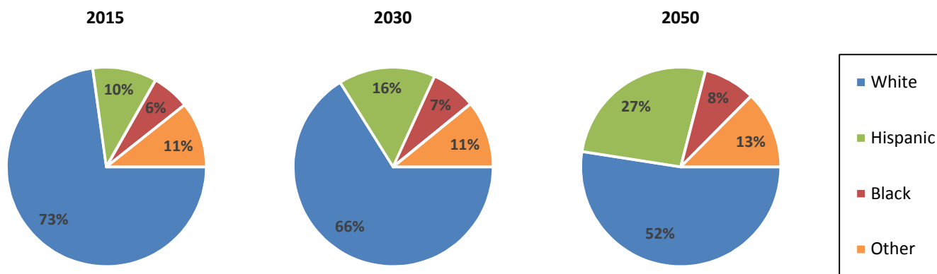
Projected Diversity of the Population Ages 65+ in Nevada, by Year
